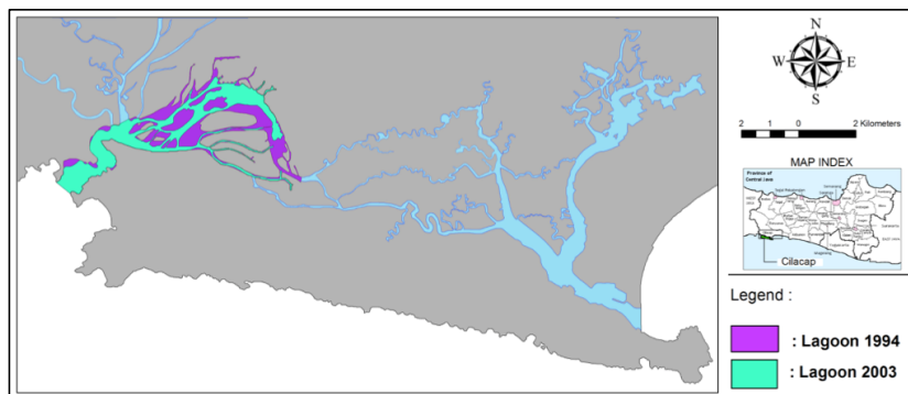
Figure 2. Changes to the lagoon's morphology (1994-2003)
