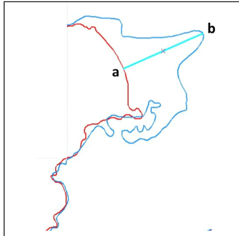
Figure 10. Coastlines changes 1978-2013 in the West Channel (A) sample area (Source: Author's own results, 2014; after MSS, TM, ETM and Landsat 8 images map, System coordinates WGS 1984 zone 49s)
