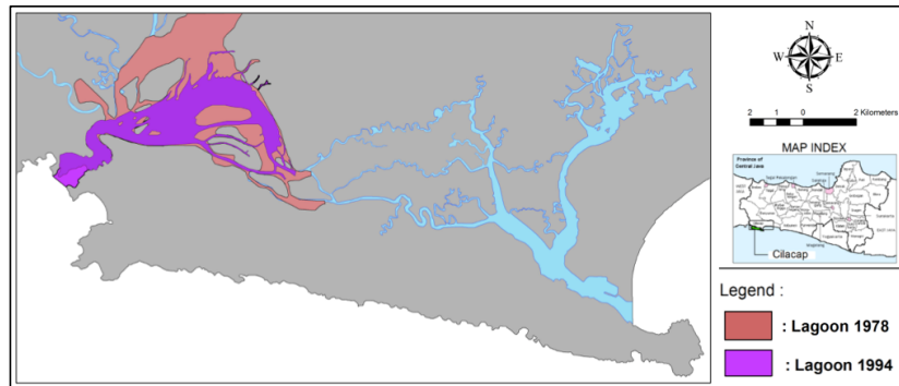
Figure 1. Changes to the lagoon's morphology (1978-1994)
